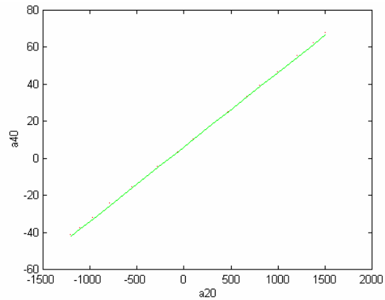
Fig. 2 Spherical aberration as a function of defocus for the f/0.7 transmission sphere used. Units are nm.
